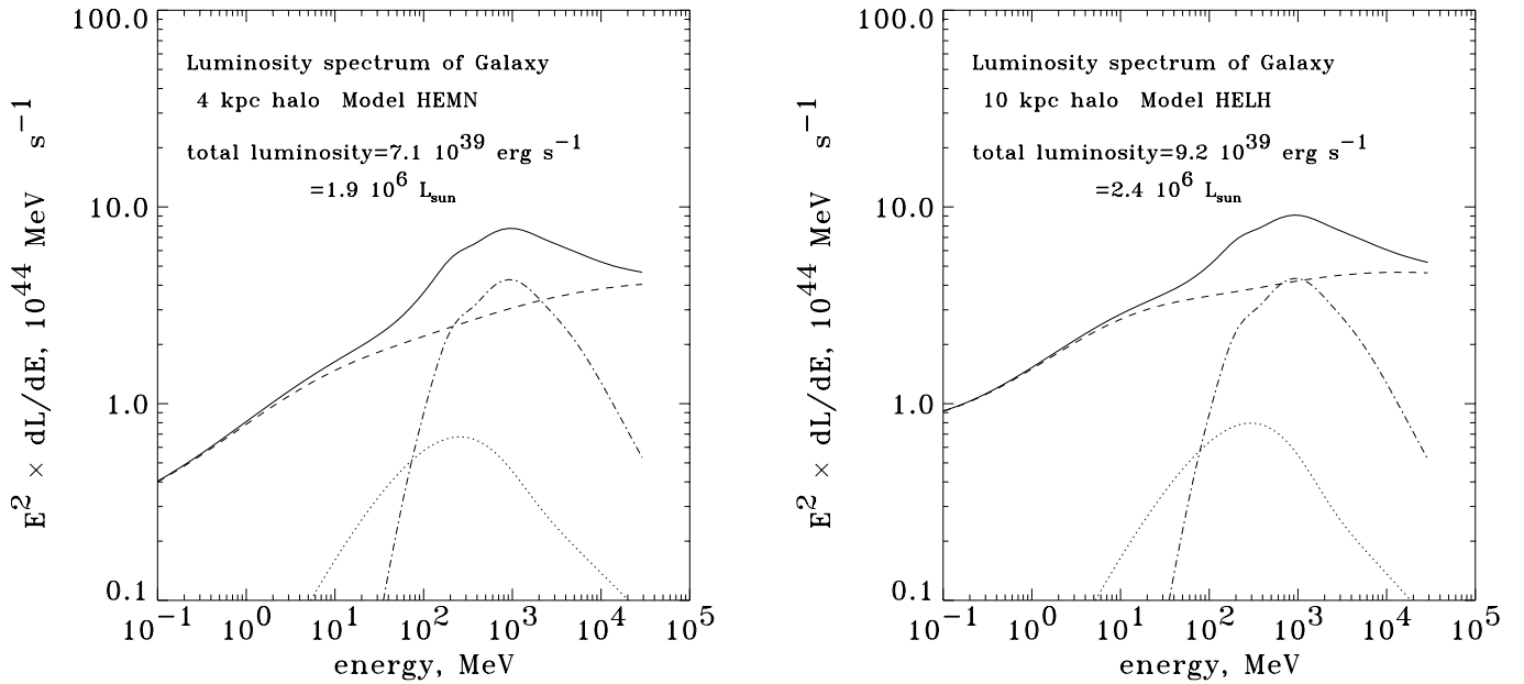
FIG. 20.—Gamma-ray luminosity spectrum of diffuse emission from the whole Galaxy using HEMN model (left), and HELH model (right). Total is shown as solid line. Separate components: IC (dashed line), bremsstrahlung (dotted line), and \pi^0 -decay (dash-dotted line).
