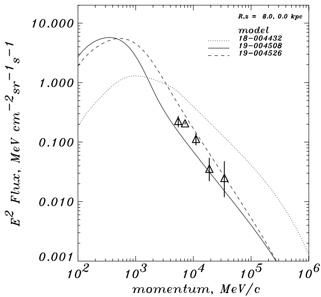
FIG. 10.—Interstellar positron spectra for models compared with data: solid line, model C; dotted line, HN; dashed line, HEMN. Data (direct measurements): HEAT experiment (Barwick et al. 1998).
