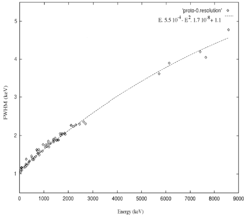
Figure 5 - The measured energy resolution of an individual SPI detector. This was measured using laboratory detectors. The resolution of the full instrument with all 19 detectors is slightly lower than this.
