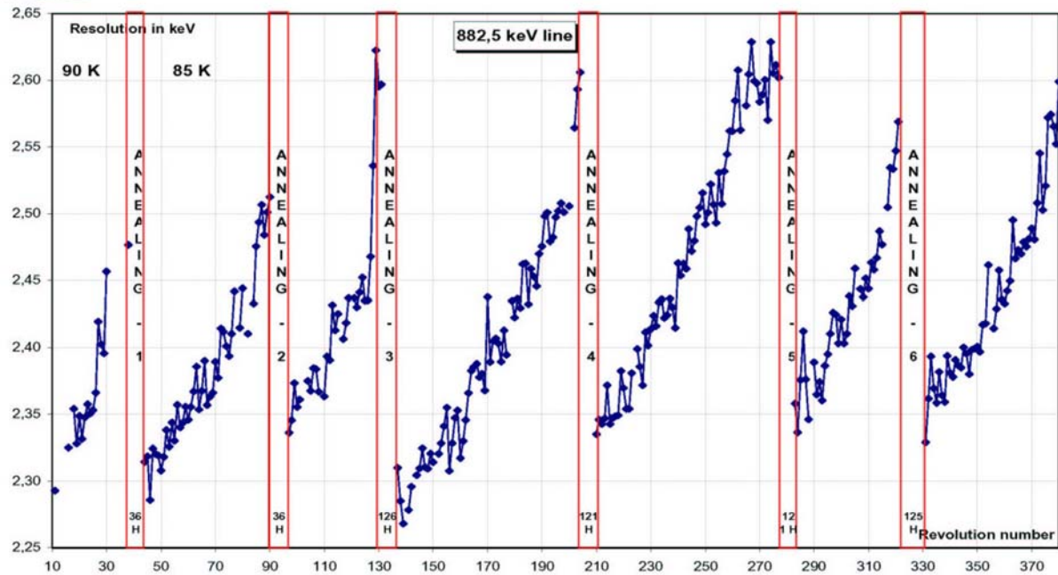
Figure 9 - The evolution of energy resolution at 882.5 keV as a function of time in-between the annealing periods.
