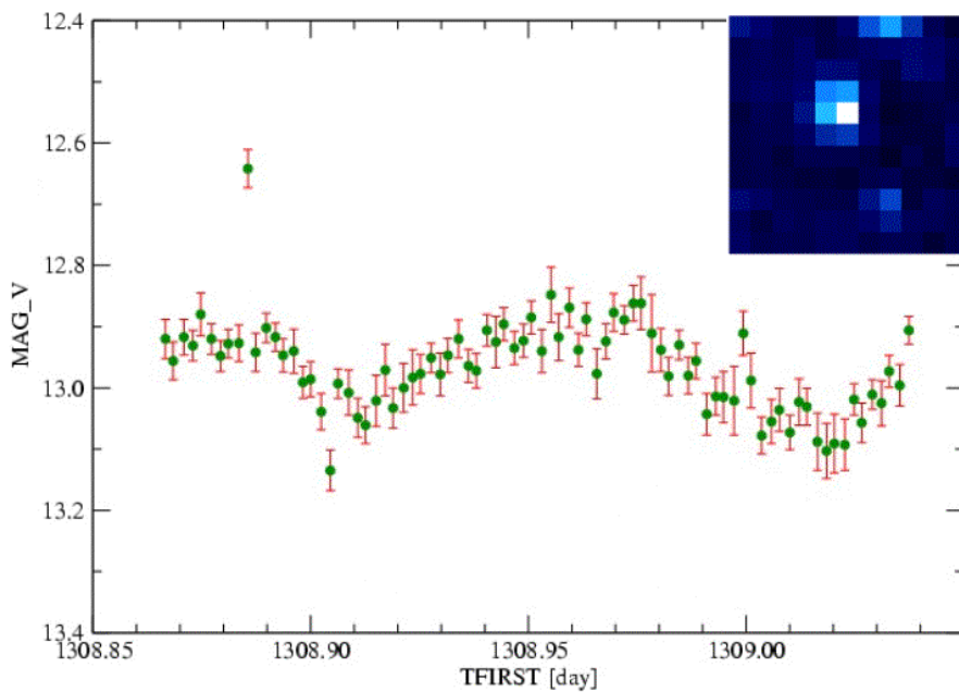
Figure 12: OMC lightcurve of the Low Mass X-ray Binary Sco X-1. It includes only single exposures of 100 seconds. The downloaded OMC sub-window for this source is also shown on the upper right corner of the graph
