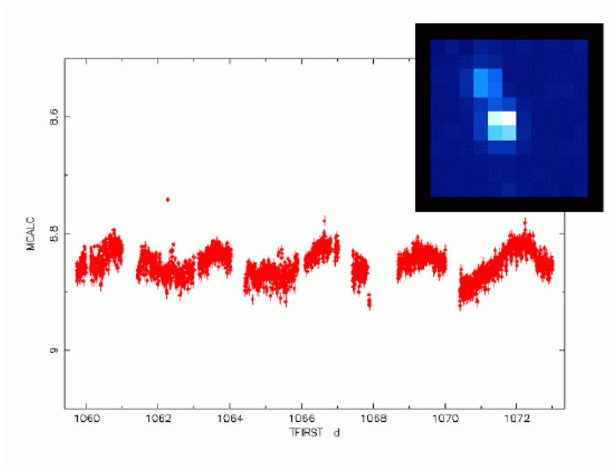
Figure 11: Computed light curve for Cyg X-1 using single exposures of 10 and 30 seconds. The OMC sub-window for Cyg X-1 is shown on the upper right corner of the graph.
