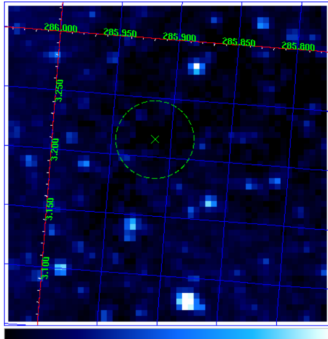
Figure 4: This image corresponds to the High Mass X-ray Binary 4U 1901+03, which generated a mosaic of 5 \times 5 OMC sub-windows ( 16' \times 16' ). The green cross and circle are the position and error of 4U 1901+03 in the IBIS catalogue, respectively.
