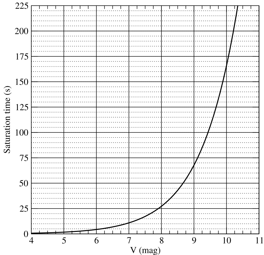
Figure 9: CCD saturation time as a function of V magnitude. Note that for integrations of 50 s, all stars with m_V > 8.6 will saturate the CCD. For the shortest OMC integration times, the brightest stars that can be observed should be fainter than m_V > 4-5 .
