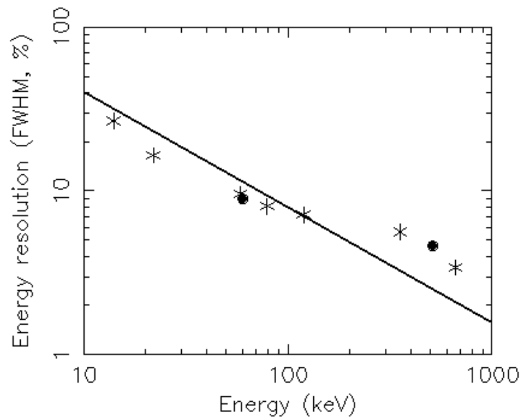
Figure 12. The energy resolution of ISGRI. Solid line: theoretically expected values; points (stars): values measured before launch using an engineering model. The study of the in-flight W fluorescence line at 60 keV and the e^+e^- annihilation lines at 511 keV (shown as filled circles) do not reveal any evidence of a change of the ISGRI spectral performance.
