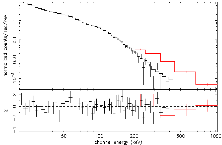
Figure 8. Crab photon spectrum together with the fit to a power-law emission model, dN/dE = 0.54 \times 10^{-3} (E/100 \text{ keV})^{-2.22} photons \text{cm}^{-2} \text{ s}^{-1} \text{ keV}^{-1} . Based on ISGRI data collected during an on-axis staring observation in revolutions 102 and 103, with a total net exposure time of 50 ksec, and PICsIT data collected in revolutions 39-45, with a total net exposure time of 625 ksec. The data were analysed using OSA version 5, and a systematic error of 1% and 5% has been added to each spectral bin of ISGRI and PICsIT, respectively. The goodness-of-fit is \chi^2 = 55.2 for 57 degrees of freedom. The intercalibration constant between ISGRI (set as reference) and PICsIT is 0.64 \pm 0.05 .
