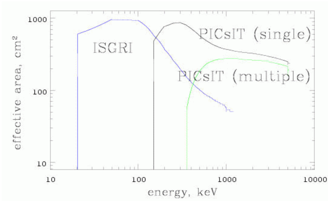
Figure 1: Effective area of the IBIS instruments ISGRI and PICsIT (single and multiple events, see Section 3.1).
