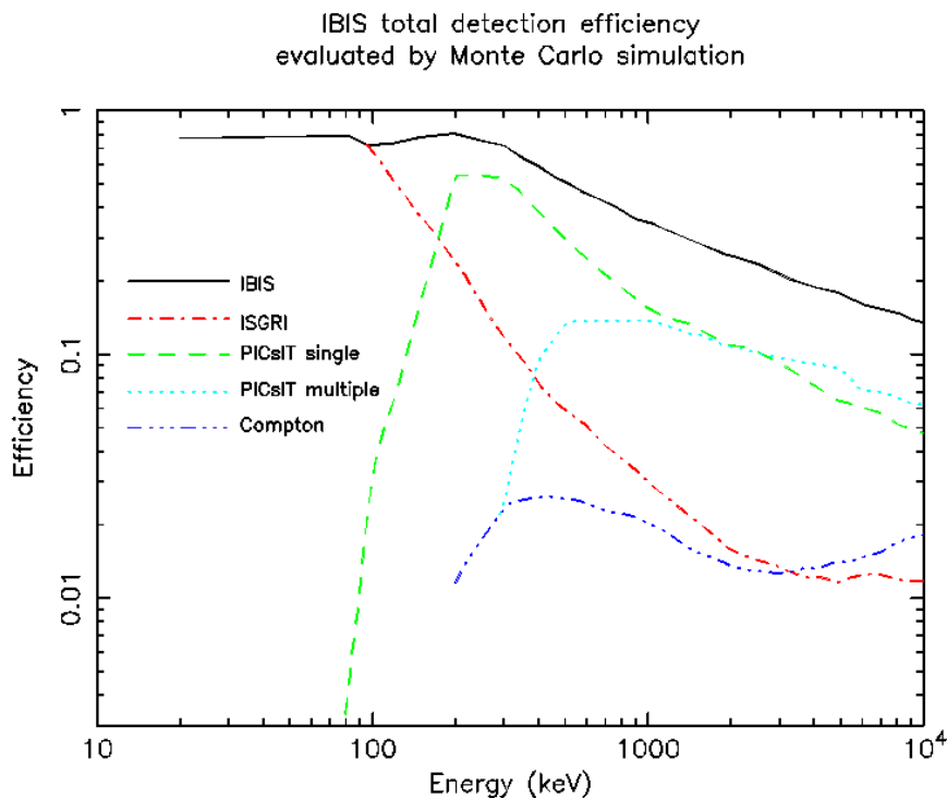
Figure 5. IBIS efficiencies for the various detection techniques, as evaluated pre-launch.
