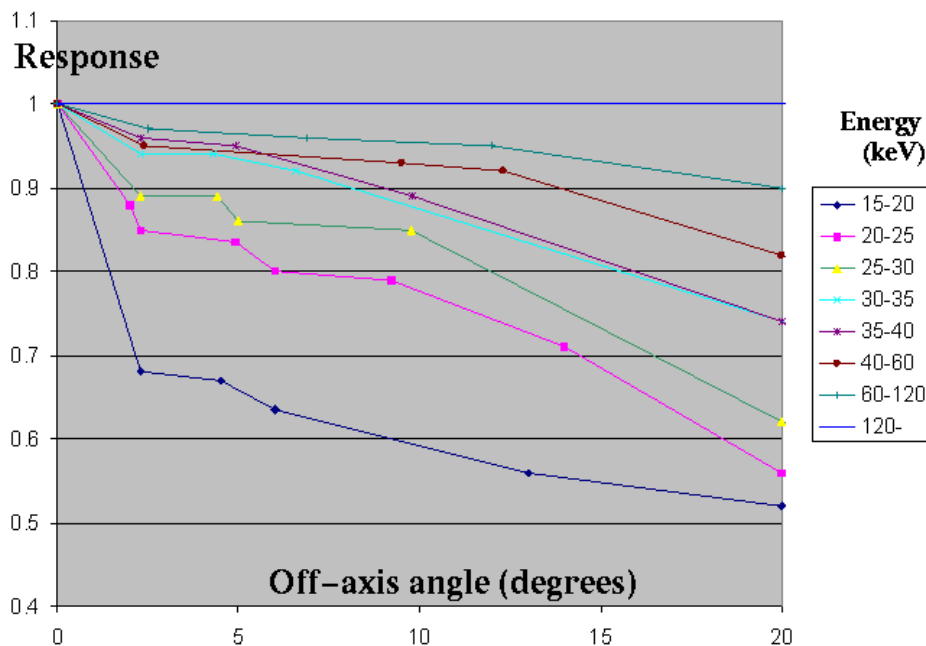
Figure 17. Deviations from the theoretical response of the IBIS telescope for various off-axis angles in different energy bands. Note that the OSA software from version 4 onwards corrects for these deviations.
