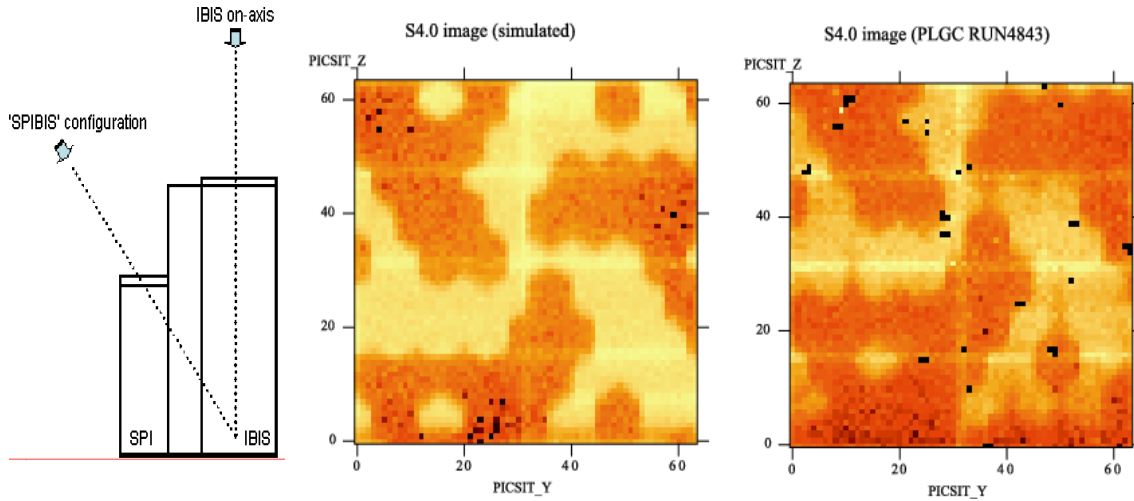
Figure 7. Left: Off-axis source positions for the SPIBIS configuration, as well as the shielding tests, during the pre-flight calibrations. Middle and right: PICsIT shadowgrams from simulations (middle) and pre-flight calibration data (right). The images are slightly offset due to the inaccuracy in the supplied source position.
